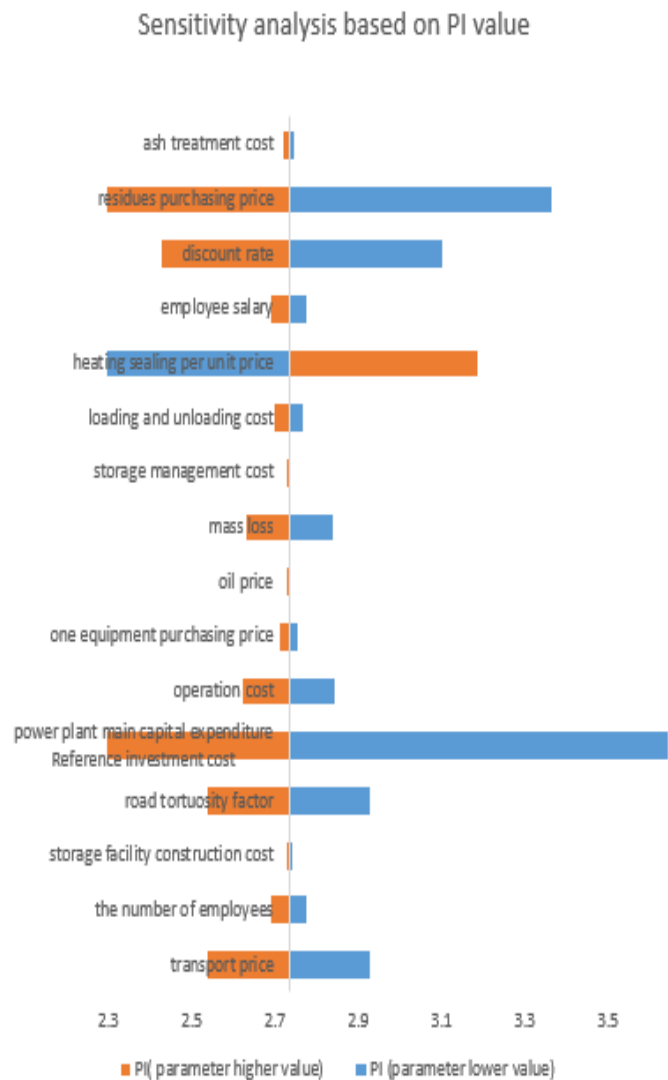
Fig 4 Sensitivity analysis for scenario 2.
